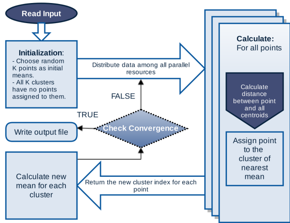
Fig. 1: K-Means parallel implementation
